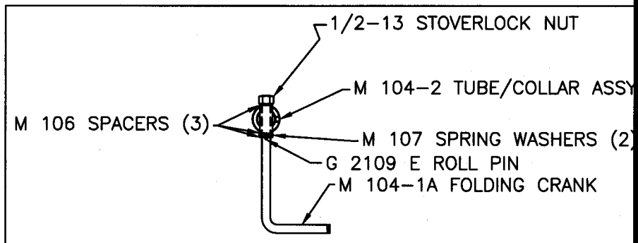
FOLDING CRANK - PARTS DETAIL M 104 A
